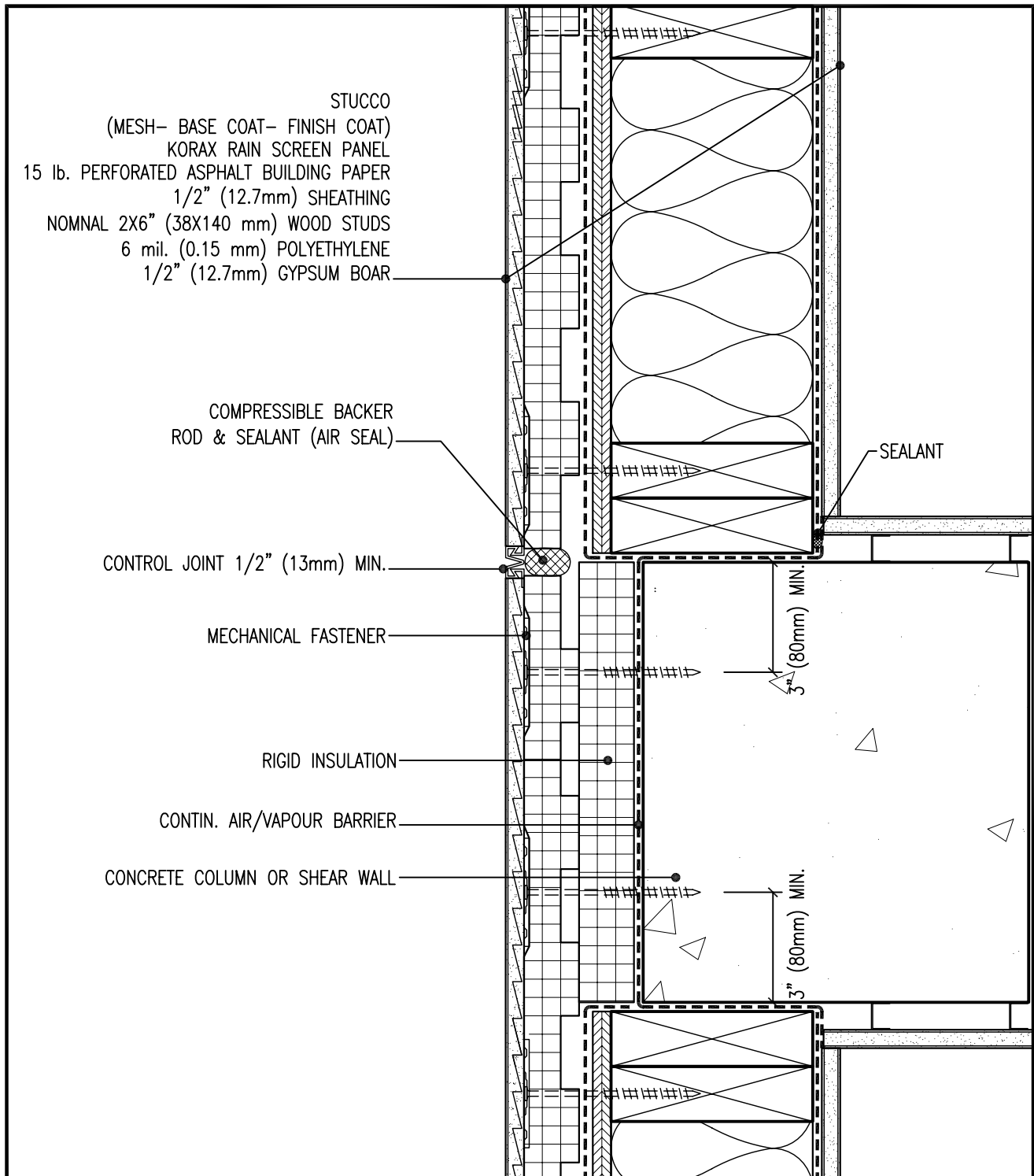
Stucco \ Wood Stud Wall Plan Detail @ Control Joint
