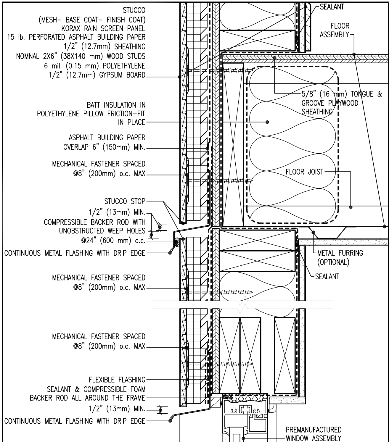
Stucco \ Wood Stud Wall Detail @ Window Head Aluminum Window
