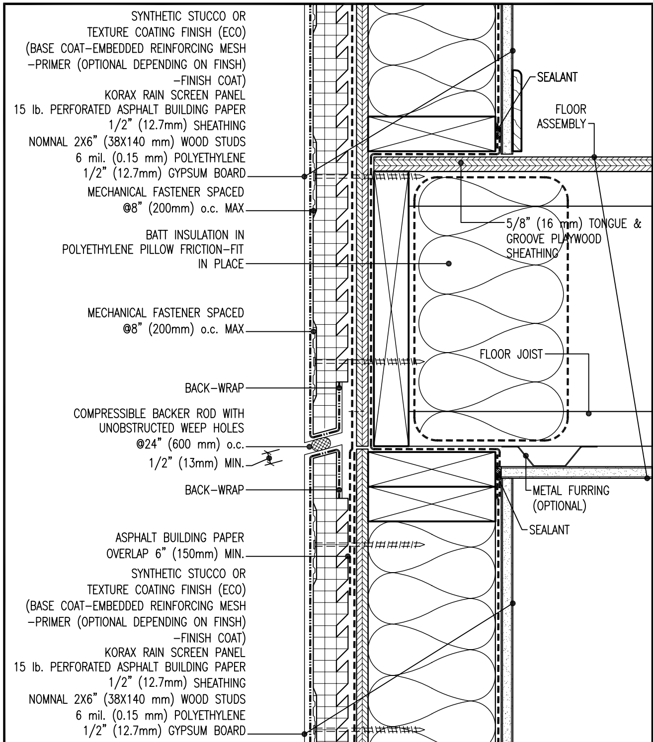
Synthetic Stucco or Texture Coating \ Wood Stud Wall Detail @ Floor
