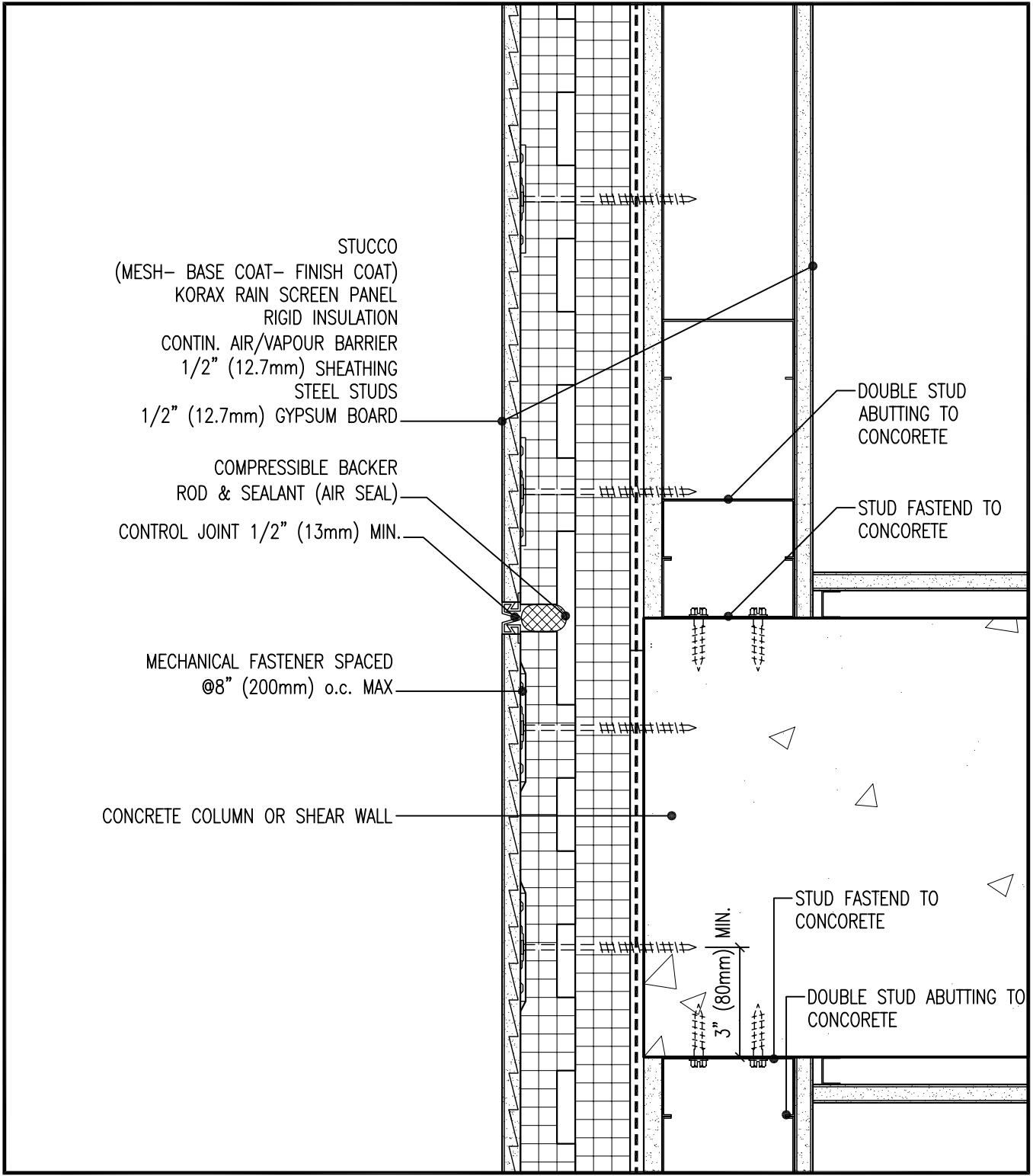
Stucco \ Steel Stud Wall Plan Detail @ Control Joint
