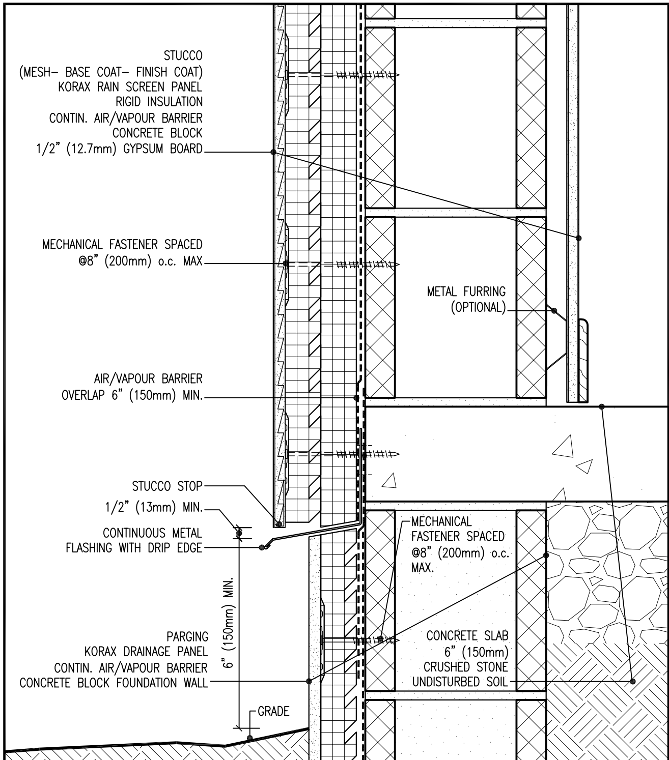
Stucco \ Concrete Block Wall Detail @ Foundation Concrete Block Foundation Wall
