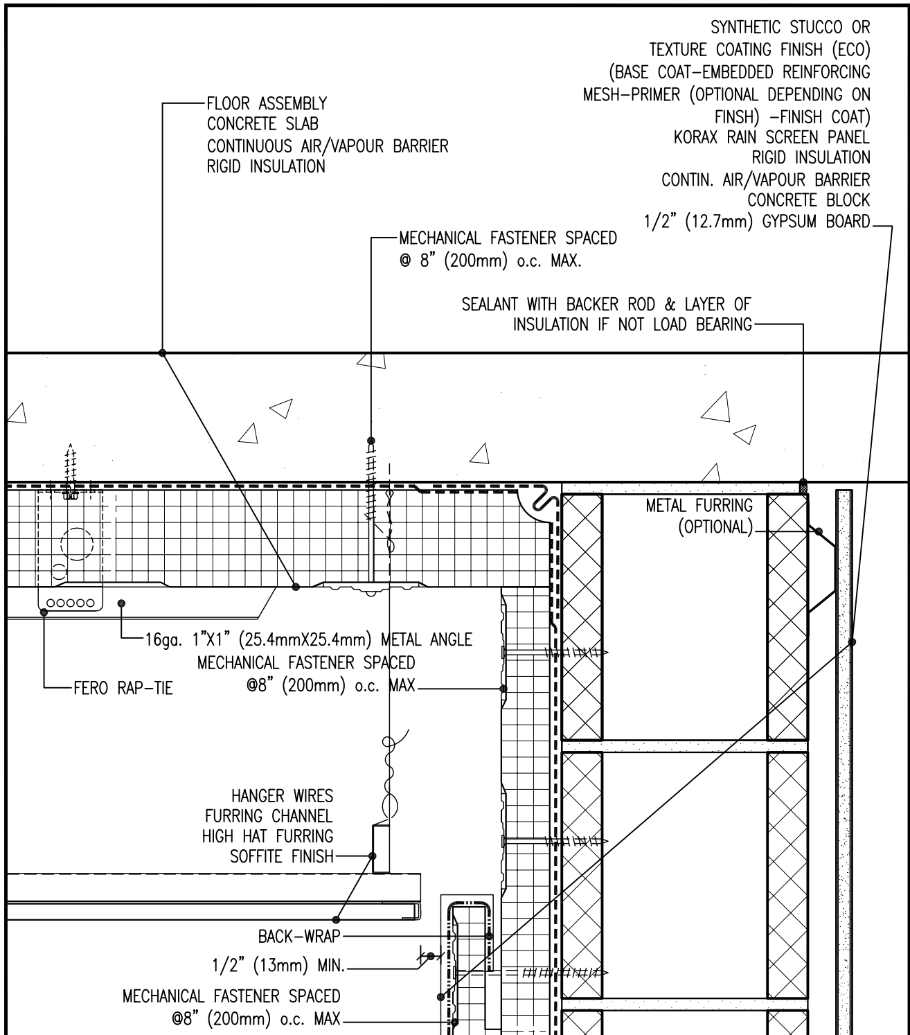
Synthetic Stucco or Texture Coating \ Concrete Block Wall Detail @ Cantilevered Floor Slab Cold Soffit
