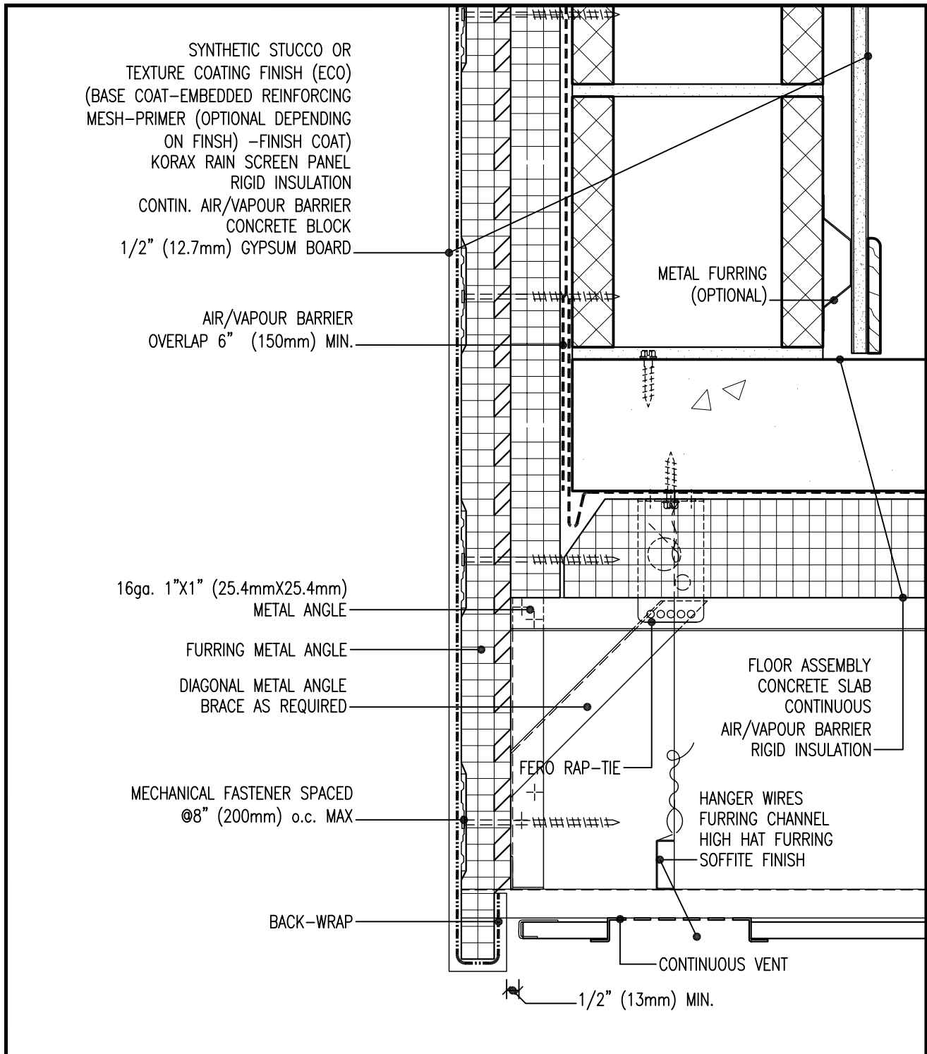
Synthetic Stucco or Texture Coating \ Concrete Block Wall Detail @ Cantilevered Floor Slab Edge Cold Soffit
