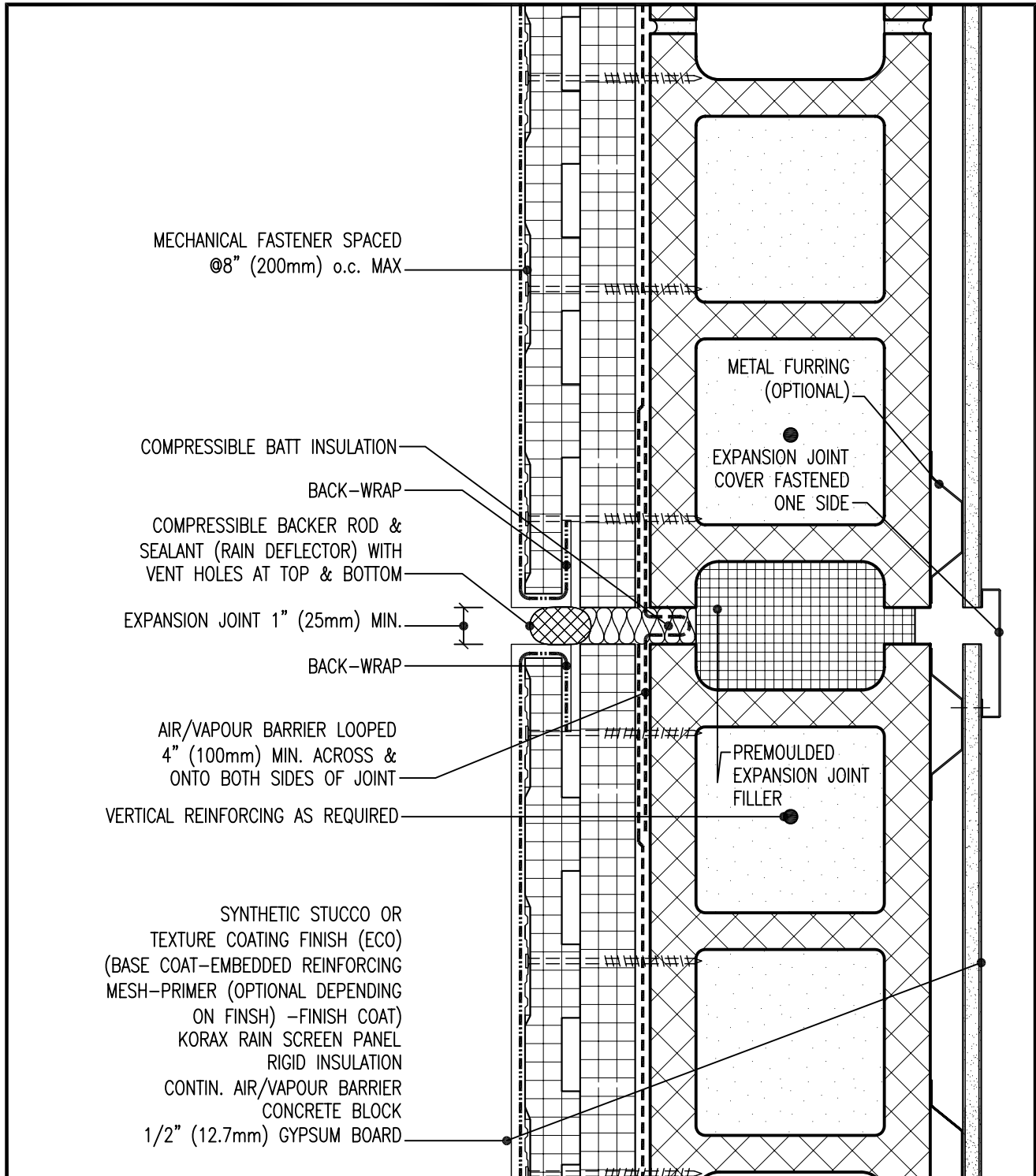
Synthetic Stucco or Texture Coating \ Concrete Block Wall Plan Detail @ Structural Expansion Joint
