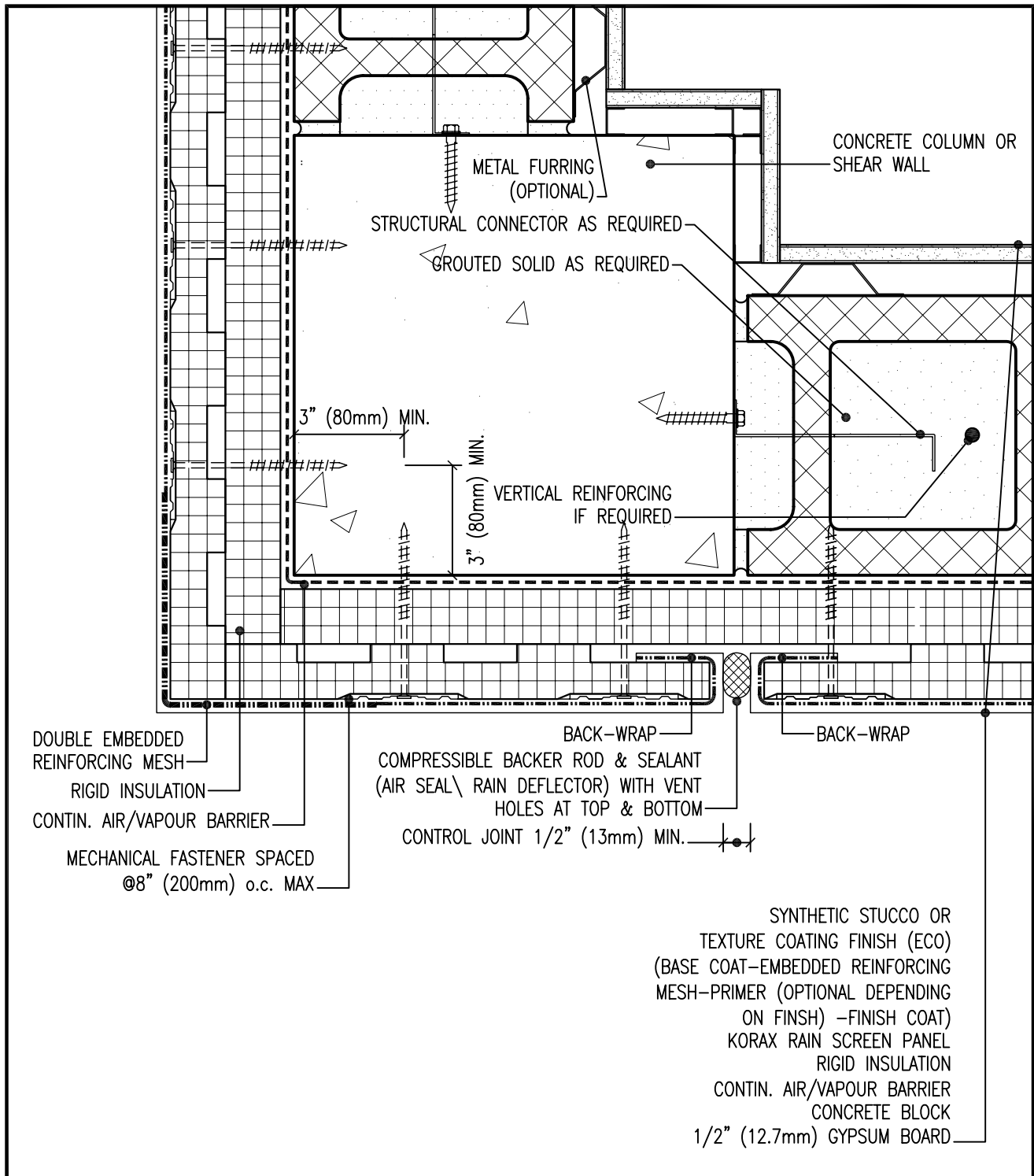
Synthetic Stucco or Texture Coating \ Concrete Block Wall Plan Detail @ Corner \ Control Joint
